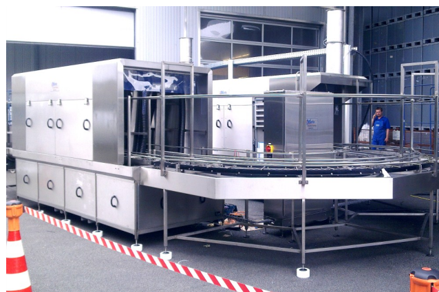
Washing machine Mafo 450MBH with Mafo 470MBHA Blow-Off For pallet boxes.
